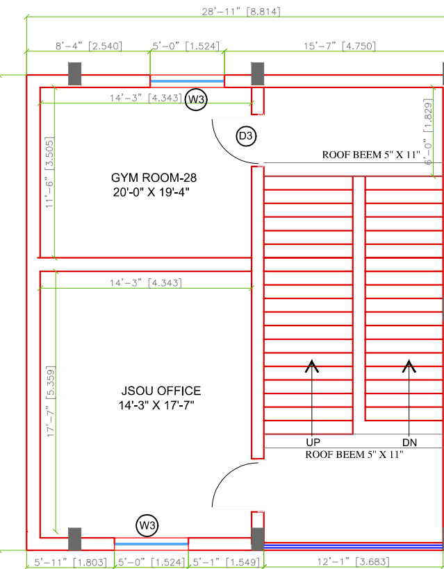
BUILDING NO -01 GROUND FLOOR
