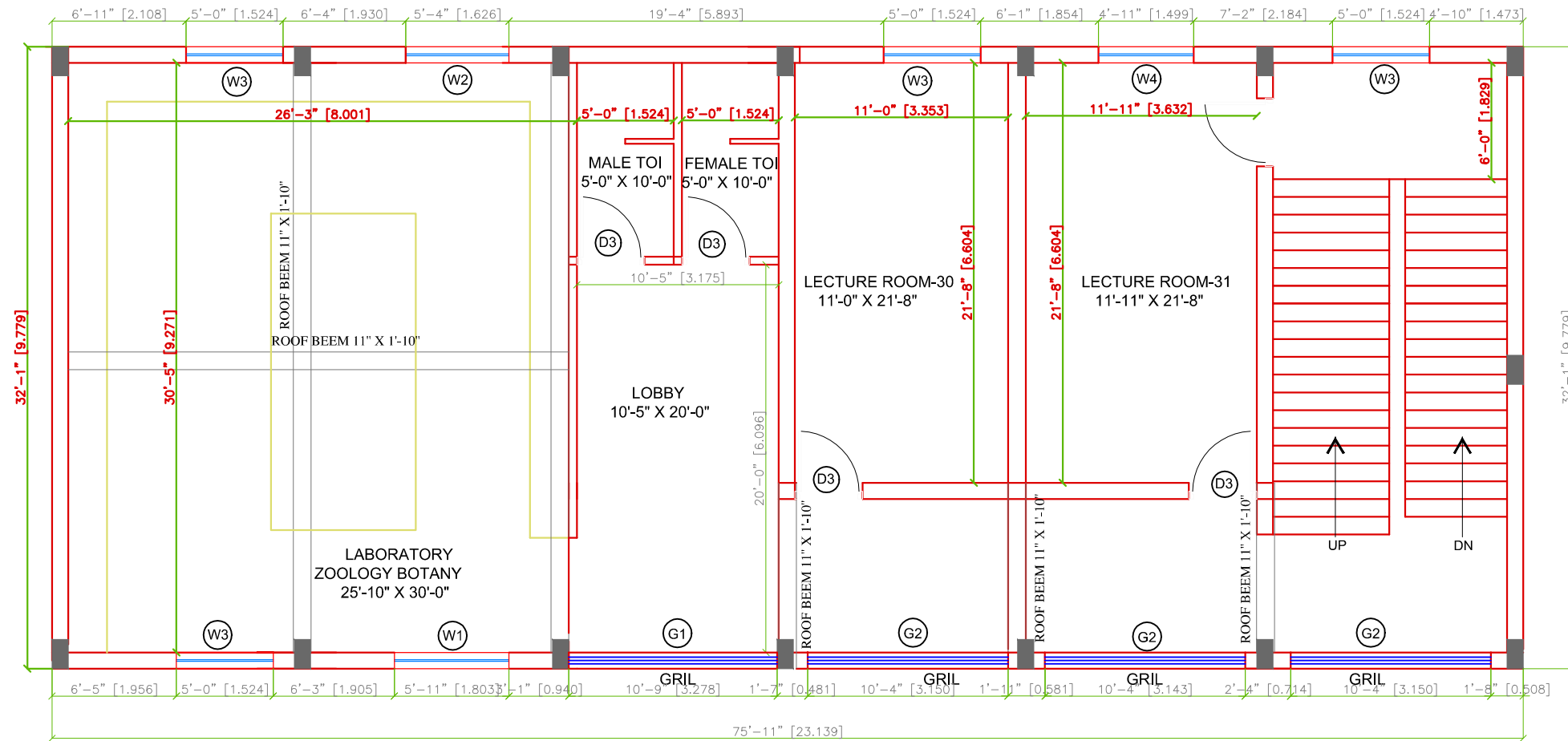
BUILDING NO -01 FRIST FLOOR
